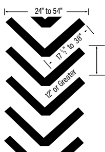
1" x 2" Wide Rect. Cleats for 24" or Wider Belts
